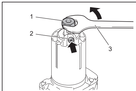
► 1. Collet nut 2. Shaft lock 3. Wrench
