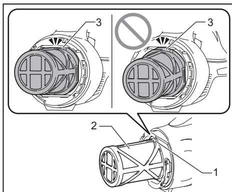
► 1. Groove of cleaner housing 2. Prefilter 3. Securing lip
