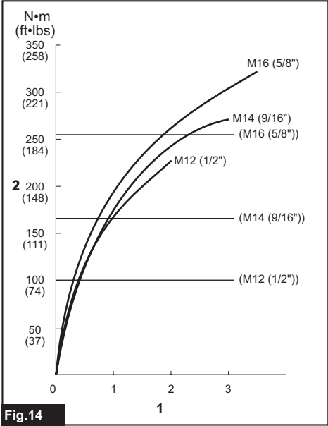
Fig.14 ► 1. Fastening time (seconds) 2. Fastening torque
