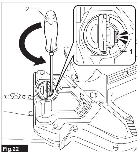
► 1. Slot 2. Slotted screwdriver
